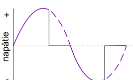
Rerewse- phase control dimmer
